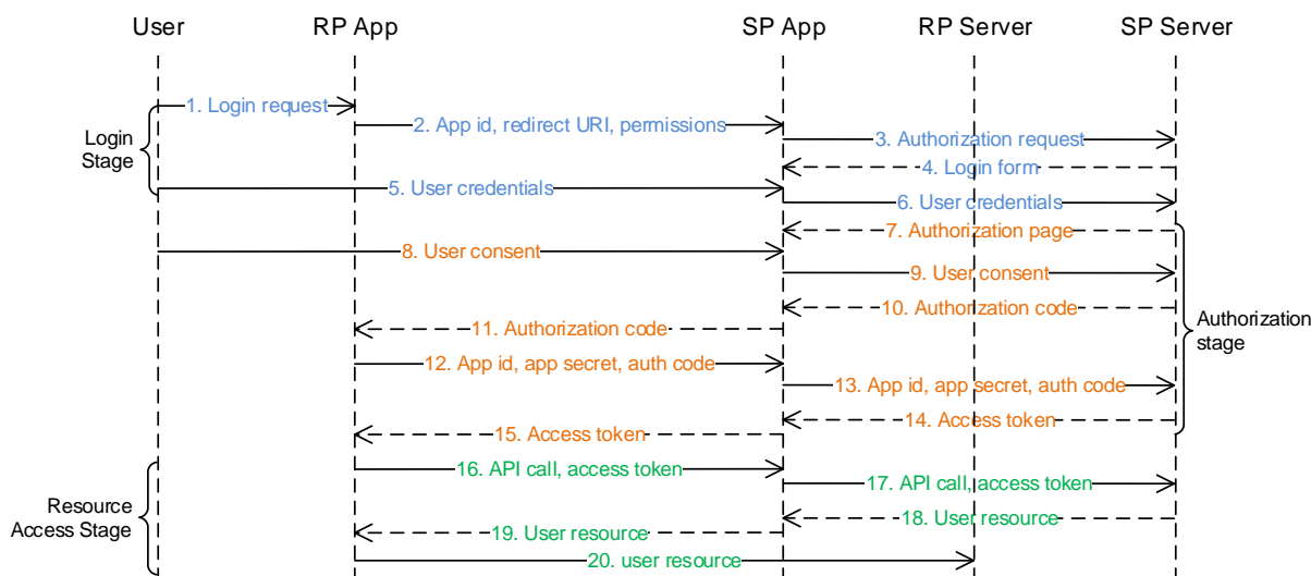
Figure 2: Model of OAuth authentication with SP app as the user-agent
